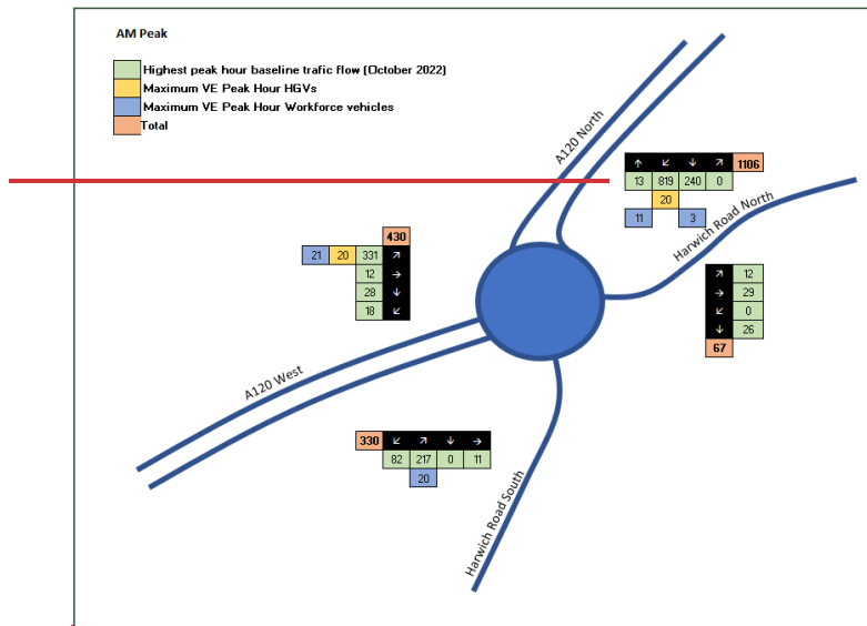
Figure 6-4: Forecast Maximum Morning Peak Hour VE Construction Vehicle Movements at the A120/ Harwich Road Roundabout
