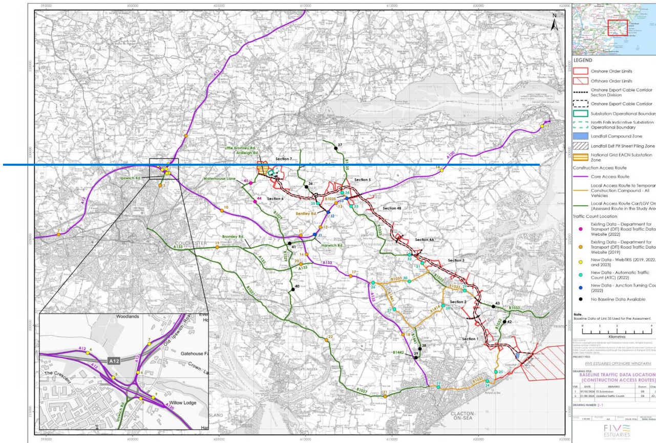
Figure 2-1: Baseline Traffic Data Locations (Construction Access Routes)
